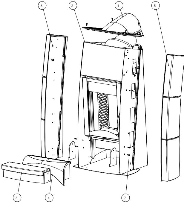
Fig. 6: Cladding components
