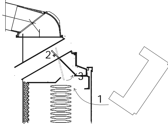
Fig. 7: Insertion of the upper baffle plate
