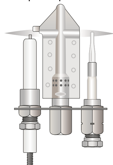
Correct position of thermocouple tip in the pilot flame
