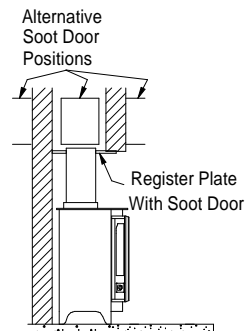
Fig. 6. Horizontal Register Plate With Top Flue Connection
