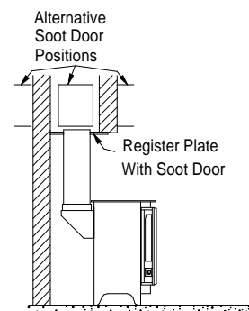
Fig. 7. Horizontal Register Plate With Optional Vertical Rear Flue Connector
