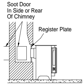
Fig. 4. Vertical Register Plate With Bricked Up Fireplace
