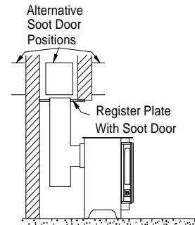
Fig. 5. Horizontal Register Plate With Rear Flue Connection
