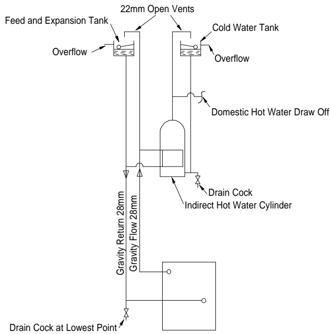
Fig. 3. Typical Gravity Hot Water System
