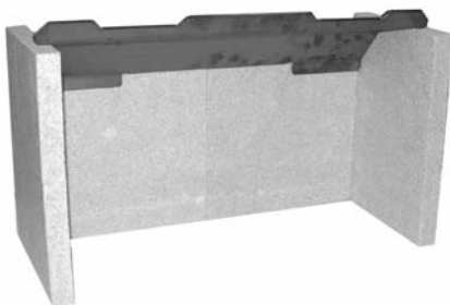
Fig. 9 Beacon multifuel liners and throat plate.
