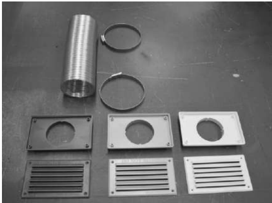
80MM \phi CCDK NEW KIT - WITH COLOURED GRILL
