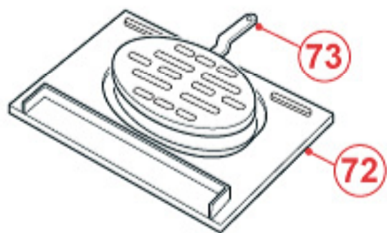
Mk3 Grate system
